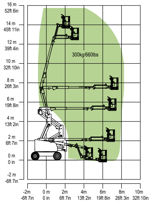
Range of Motion ZA14J
