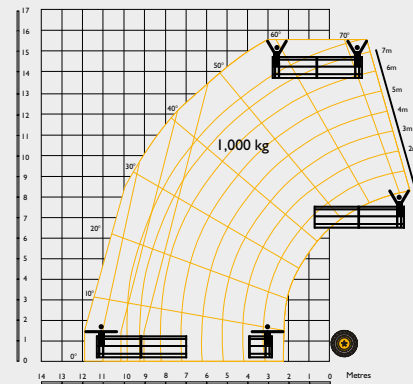
540-140 HiViz 1000kg, 180° slewing man platform, stabilisers extended
