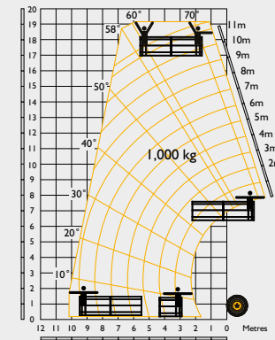
540-180 HiViz 1000kg, 180° slewing man platform, stabilisers extended
